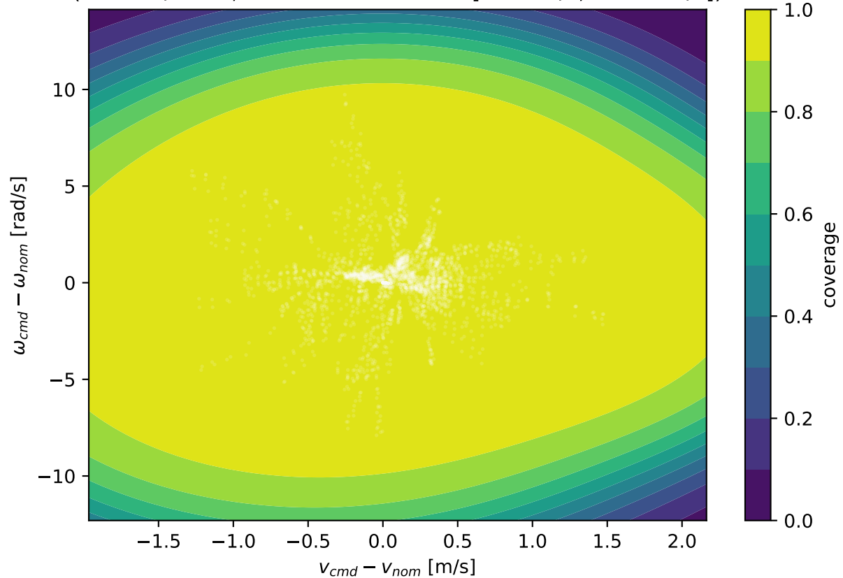
Residual coverage vs command offset (0 = off / OOD; state fixed at mean [0.74 m/s, 0.27 rad/s])
